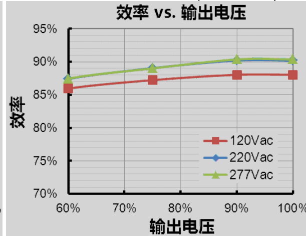
EUP-150S560ST(Io=5600mA)
