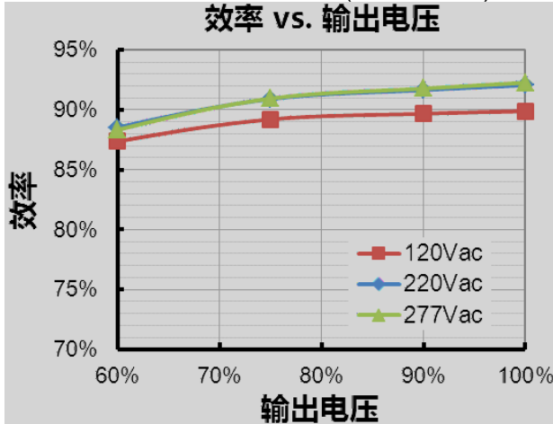
EUP-150S560ST(Io=4200mA)
