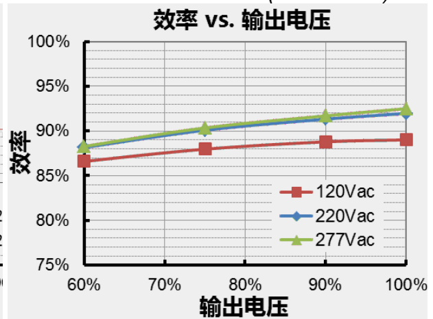
EUP-240S420ST (Io=4200mA) 效率 vs. 输出电压
