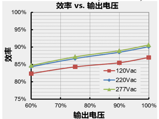
EUP-240S670ST(Io=6700mA)
