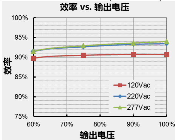
EUP-240S210ST (Io=1400mA) 效率 vs. 输出电压
