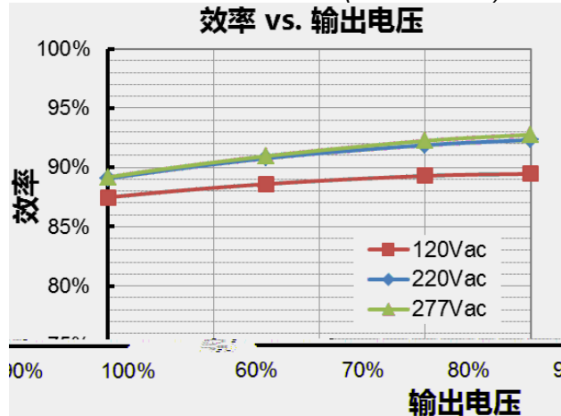
EUP-240S210ST (Io=2100mA) 效率 vs. 输出电压
